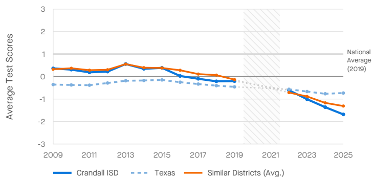
Trend in Reading Scores (All Students)
