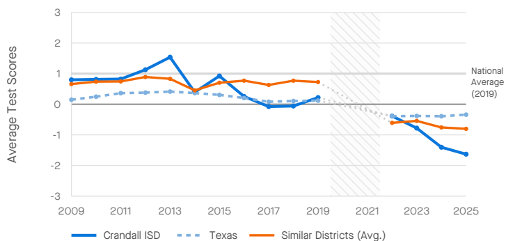
Trend in Math Scores (All Students)
