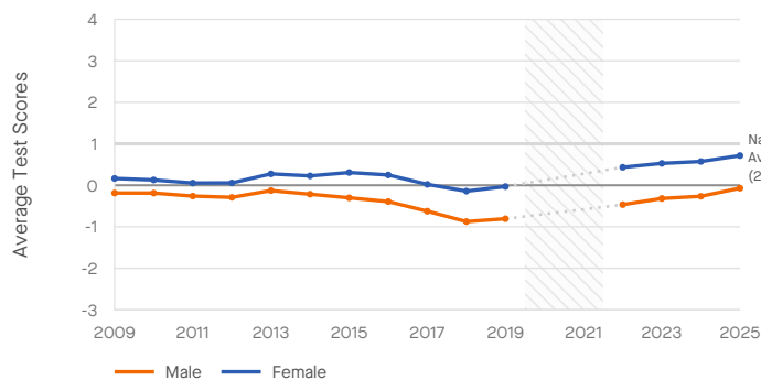
Trend in Reading Scores, by Student Gender
