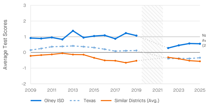
Trend in Math Scores (All Students)
